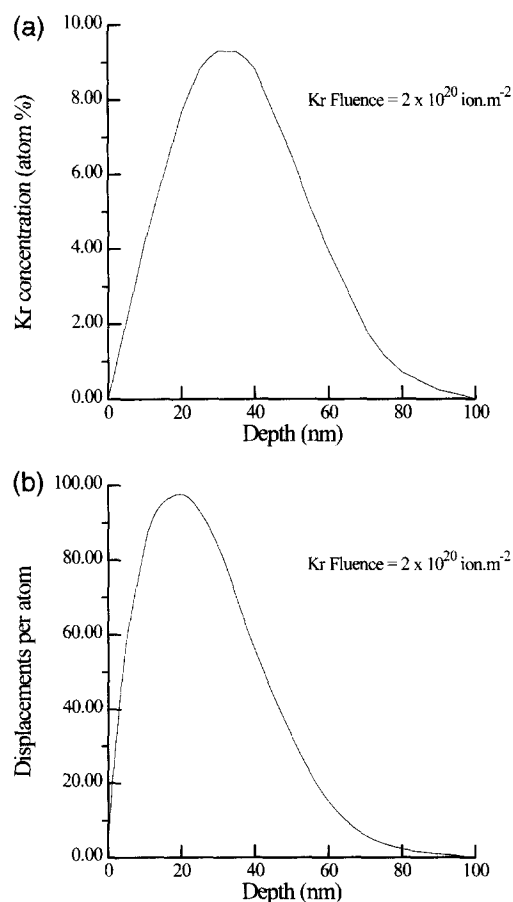
Fig. 1. (a) Concentration profile of implanted Kr atoms and (b) displacement profile in Zr, after 100 keV Kr irradiation to 2 \times 10^{20} ion m -2 as calculated by TRIM [24].
