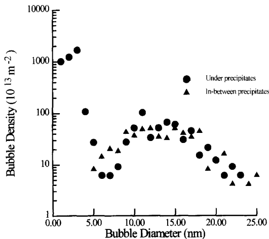
Fig. 10. Bubble size distribution in Zircaloy-4 after irradiation with 100 keV Kr ions to 2 \times 10^{20} ion m^{-2} , at 800°C. Two histograms are shown, one for under the precipitates, one for in-between. The zone under the precipitates has a high density of small bubbles.
